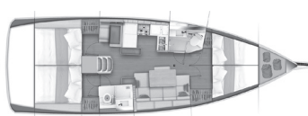
Version C 2 forward cabins 2 aft cabins / 2 heads
